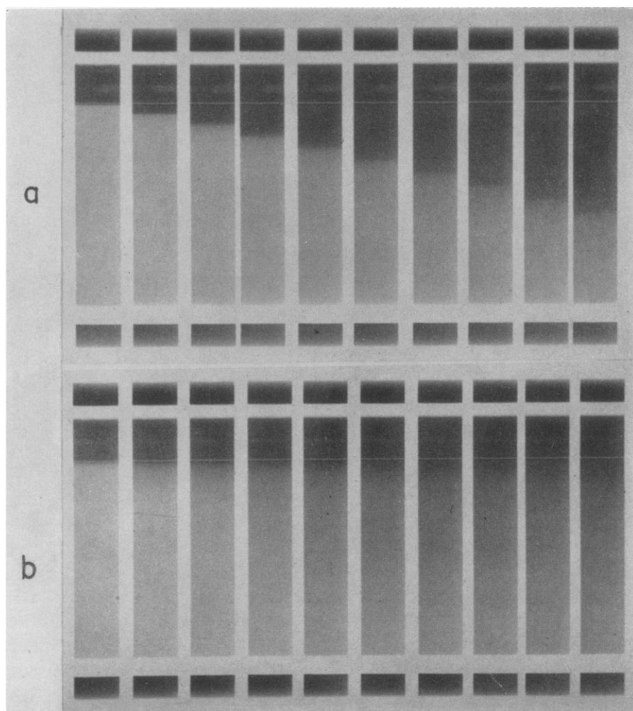
FIGURE 8 Sedimentation pattern of T 4 DNA. (a) before heating and cooling. (b) after heating and cooling.
