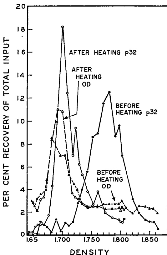
FIGURE 4 Hybrid formation in sonicated solution containing 20 \mu\text{g}/\text{ml} of non-radioactive light DNA, and 0.2 \mu\text{g}/\text{ml} of \text{P}^{32} -labeled 5-BU DNA. After heating both UV absorption and \text{P}^{32} activity are found in density range characteristic of majority light DNA.
