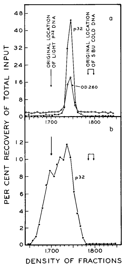
FIGURE 5 Hybrid formation in solution containing 15 \mu\text{g/ml} of light P^{32} -labeled and 15 \mu\text{g/ml} non-radioactive 5-BU DNA. (a) After heating and slow cooling P^{32} activity and UV absorption move to intermediate density. (b) Same as (a), but after sonication P^{32} activity spread from light to intermediate density.
