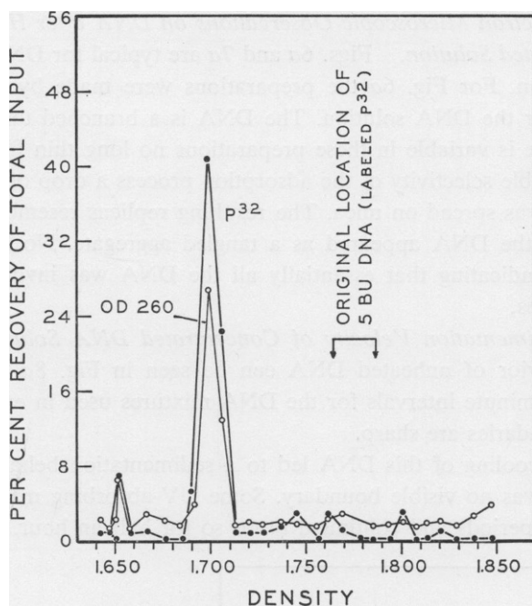
FIGURE 3 Hybrid formation in solution containing 20 \mu\text{g/ml} of non-radioactive light DNA mixed with 0.2 \mu\text{g/ml} of \text{P}^{32} -labeled 5-BU DNA. Figure shows UV absorption and \text{P}^{32} activity after heating and slow cooling.
