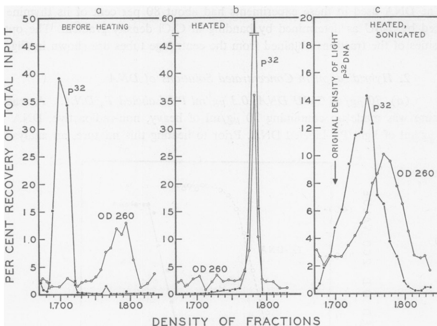
FIGURE 2 Hybrid formation in solution containing 30 \mu\text{g/ml} of non-radioactive 5-BU DNA and 0.3 \mu\text{g/ml} of light \text{P}^{32} DNA. (a) Distribution of UV-absorbing material and \text{P}^{32} activity in CsCl gradient of the mixture before heating. (b) The same mixture as in (a), but after heating and slow cooling. (c) The same as (b), but after sonication.
