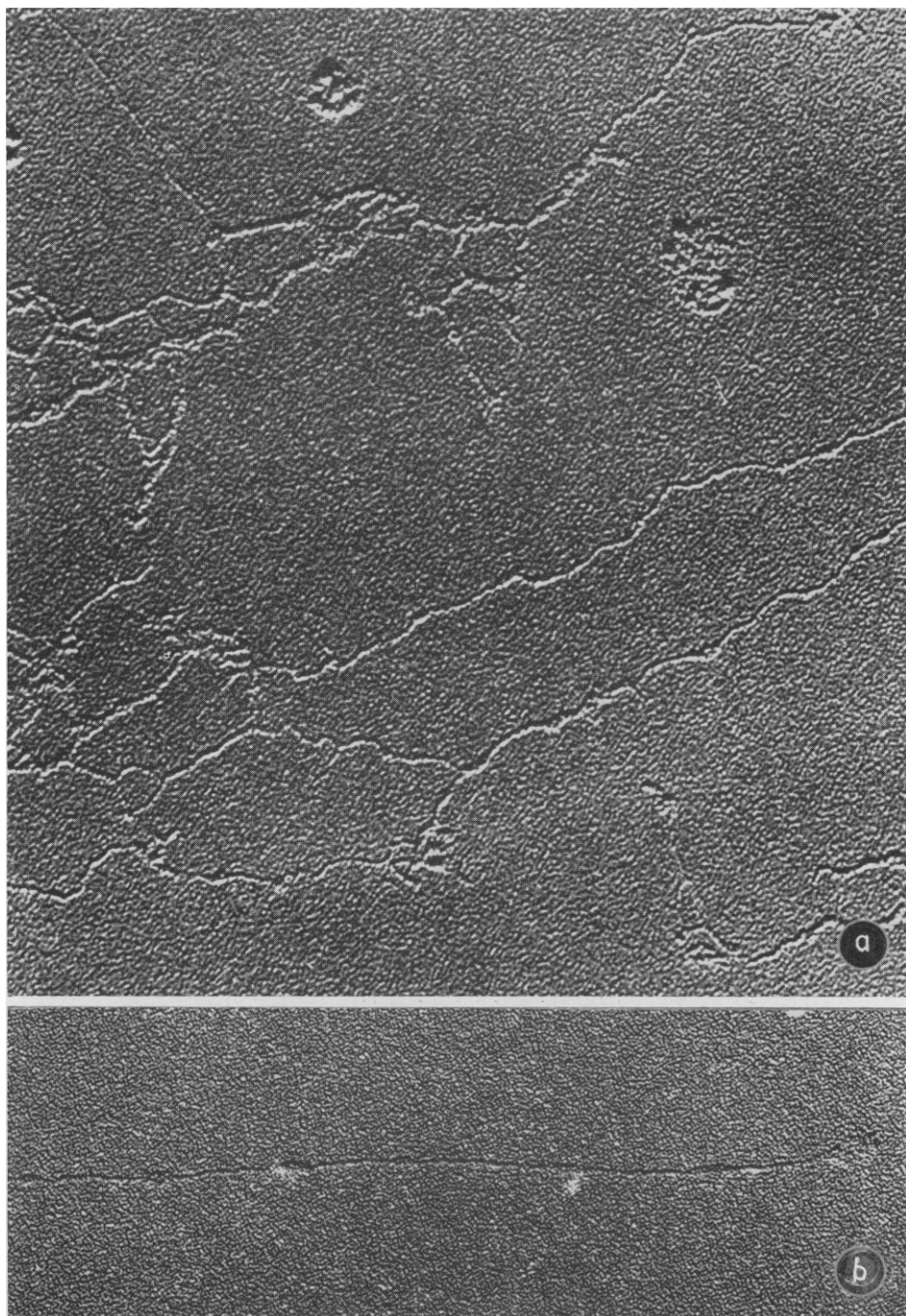
FIGURE 7 DNA spread on mica after heating and slow cooling. The concentration of DNA during heating and slow cooling was (a) 30 \mu\text{g/ml} (b) 0.6 \mu\text{g/ml} . \times 70,000 .
